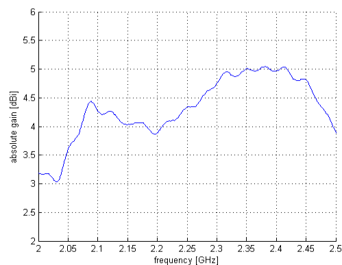
Measured gain:
